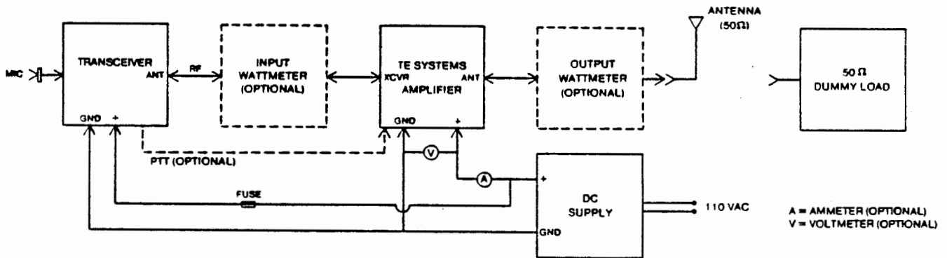
OPERATIONAL / TEST SET-UP FOR AMPLIFIER
